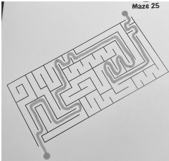
Maze 25
