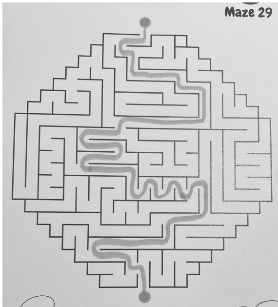
Maze 29
