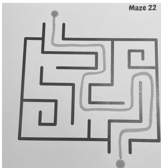
Maze 22
