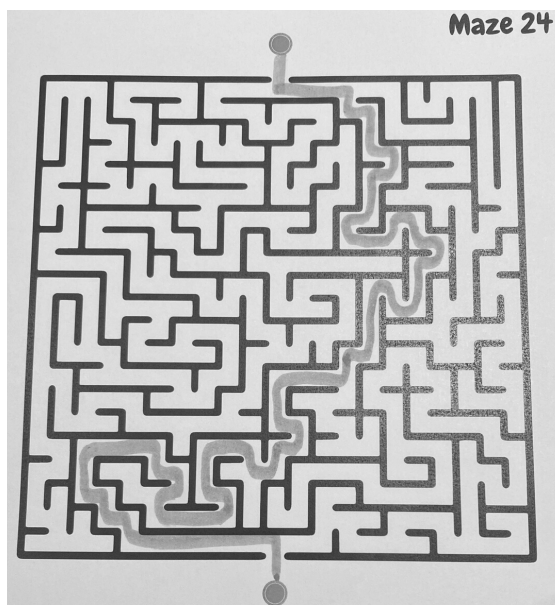
Maze 24
