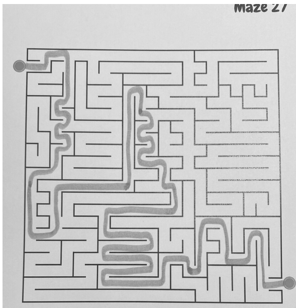
Maze 27
