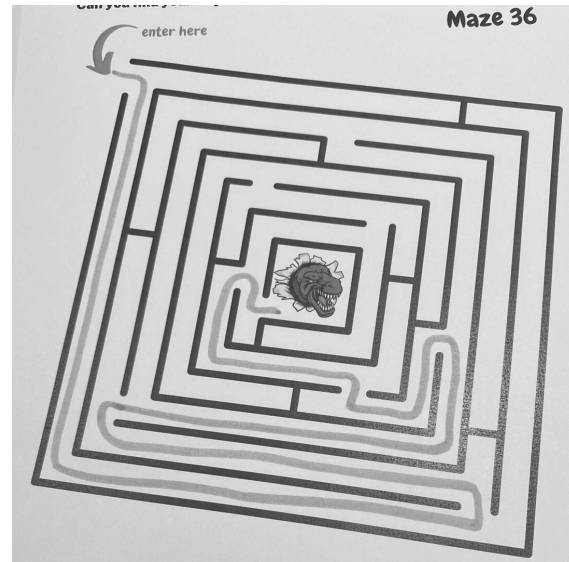
Maze 36
