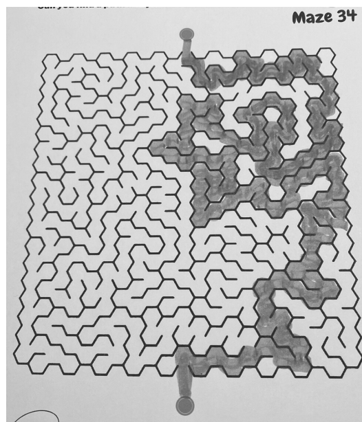
Maze 34
