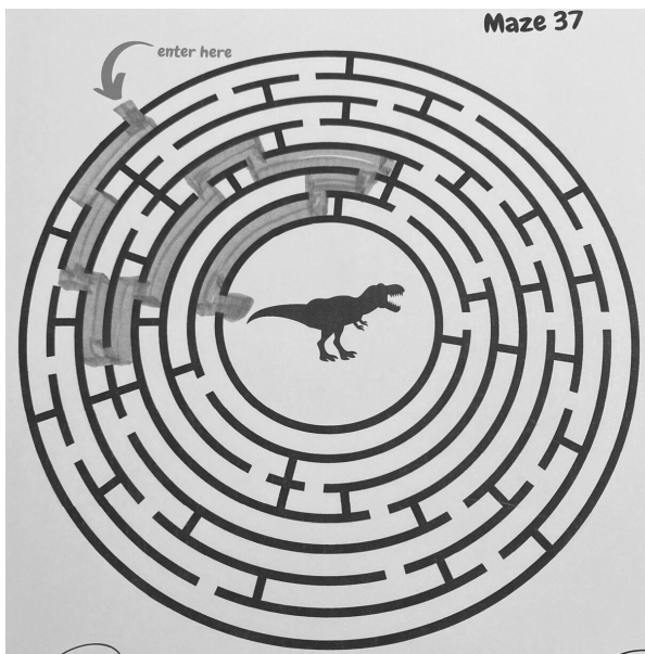
Maze 37
