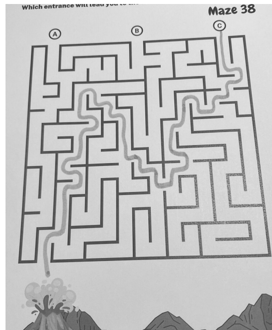
Maze 38
