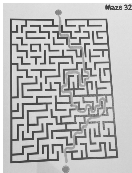
Maze 32
