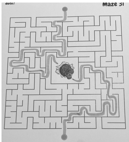
Maze 31
