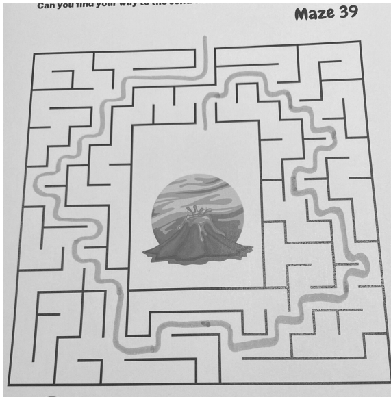
Maze 39
