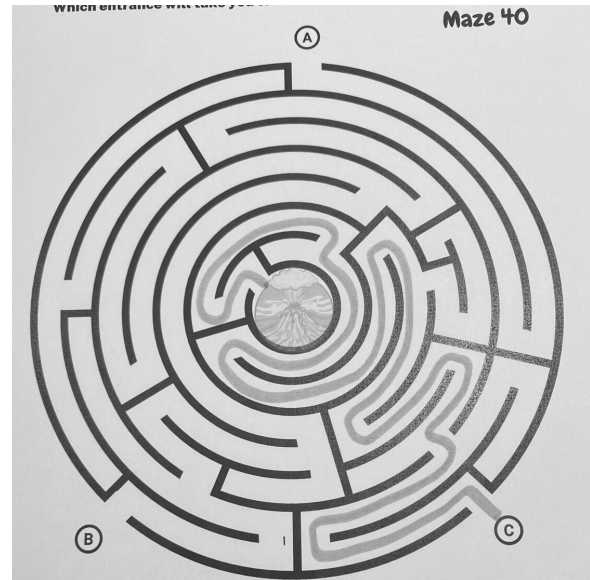
Maze 40
