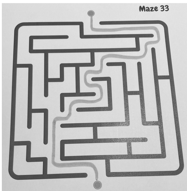
Maze 33
