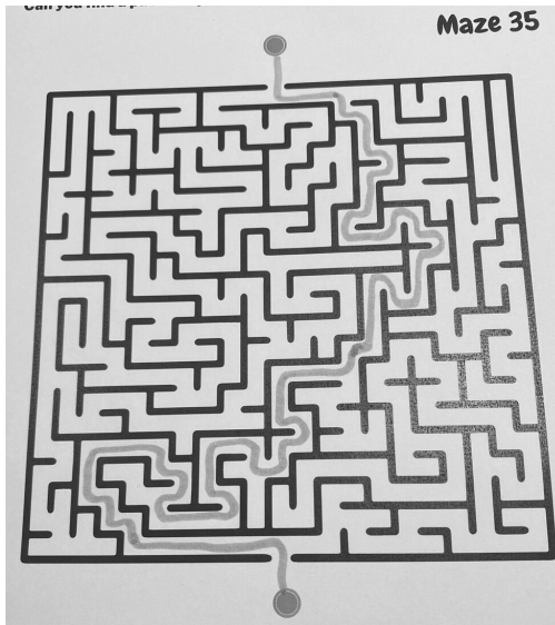
Maze 35
